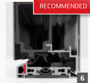
Magnet WeatherSeal sealing
